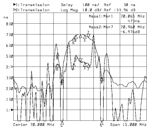
Horizontal: 1.5MHz/Div; Vertical: 1db & 10db/Div
