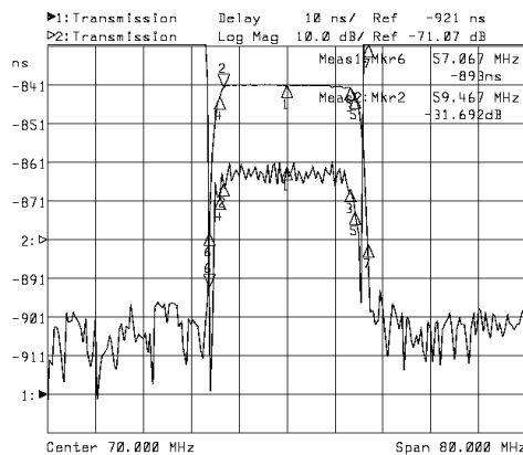
Horizontal: 8MHz/Div Vertical: 10nsec/Div
