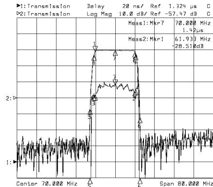
Horizontal: 8MHz/Div Vertical: 20nsec/Div
