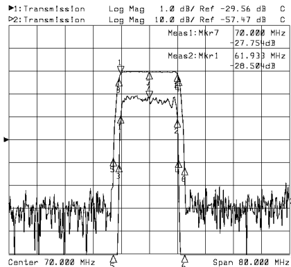
Horizontal: 8MHz/Div Vertical: 1db & 10dB/Div
