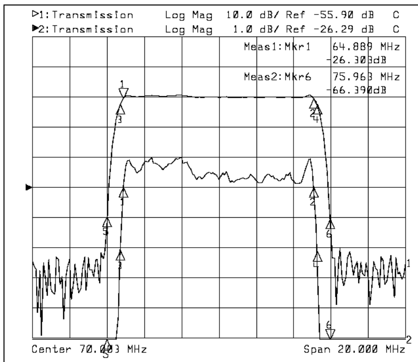
Horizontal: 2MHz/Div Vertical: 1db & 10dB/Div
