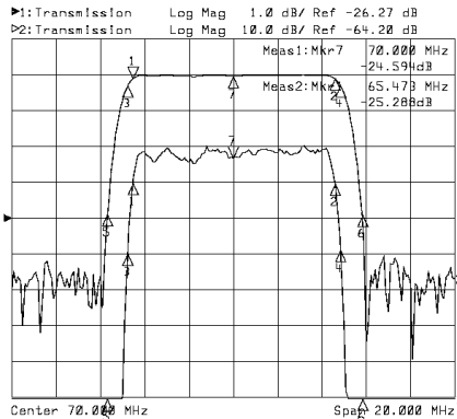
Horizontal: 2 MHz/Div Vertical: 1db & 10dB/Div
