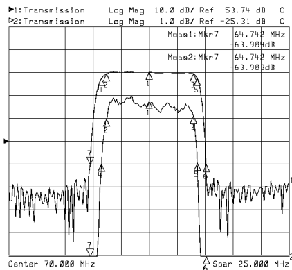
Horizontal: 2.5MHz/Div Vertical: 1db & 10dB/Div
