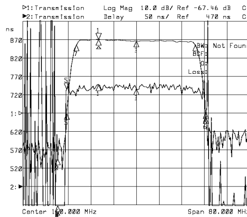
Horizontal: 8MHz/Div Vertical: 50nsec/Div
