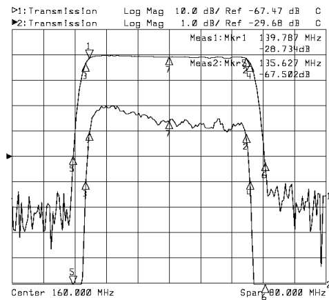
Horizontal: 8MHz/Div Vertical: 1db& 10db/Div
