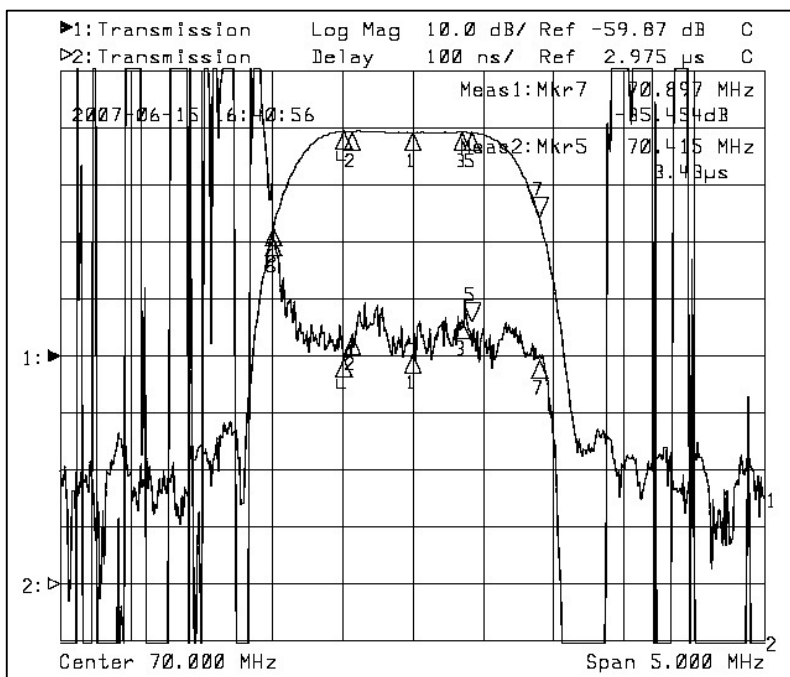
Horizontal: 0.5MHz/Div Vertical: 100ns>Div & 10dB/Div
