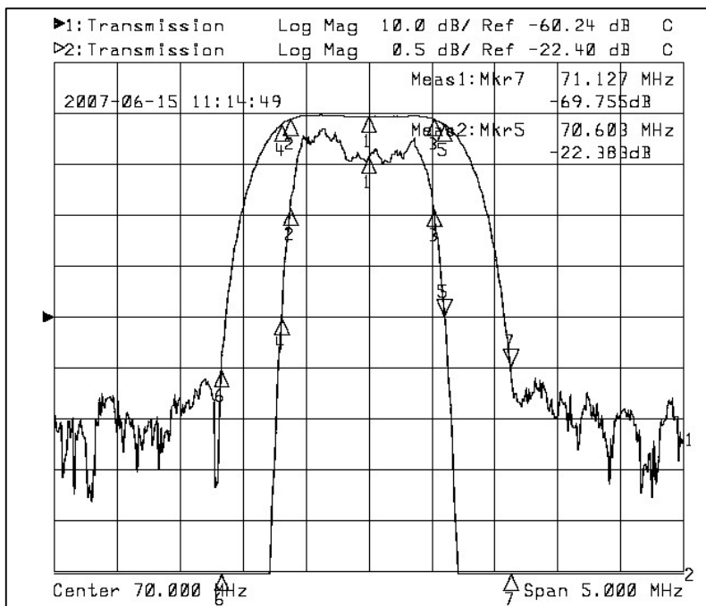
Horizontal: 0.5MHz/Div Vertical: 0.5dB/Div & 10dB Div
