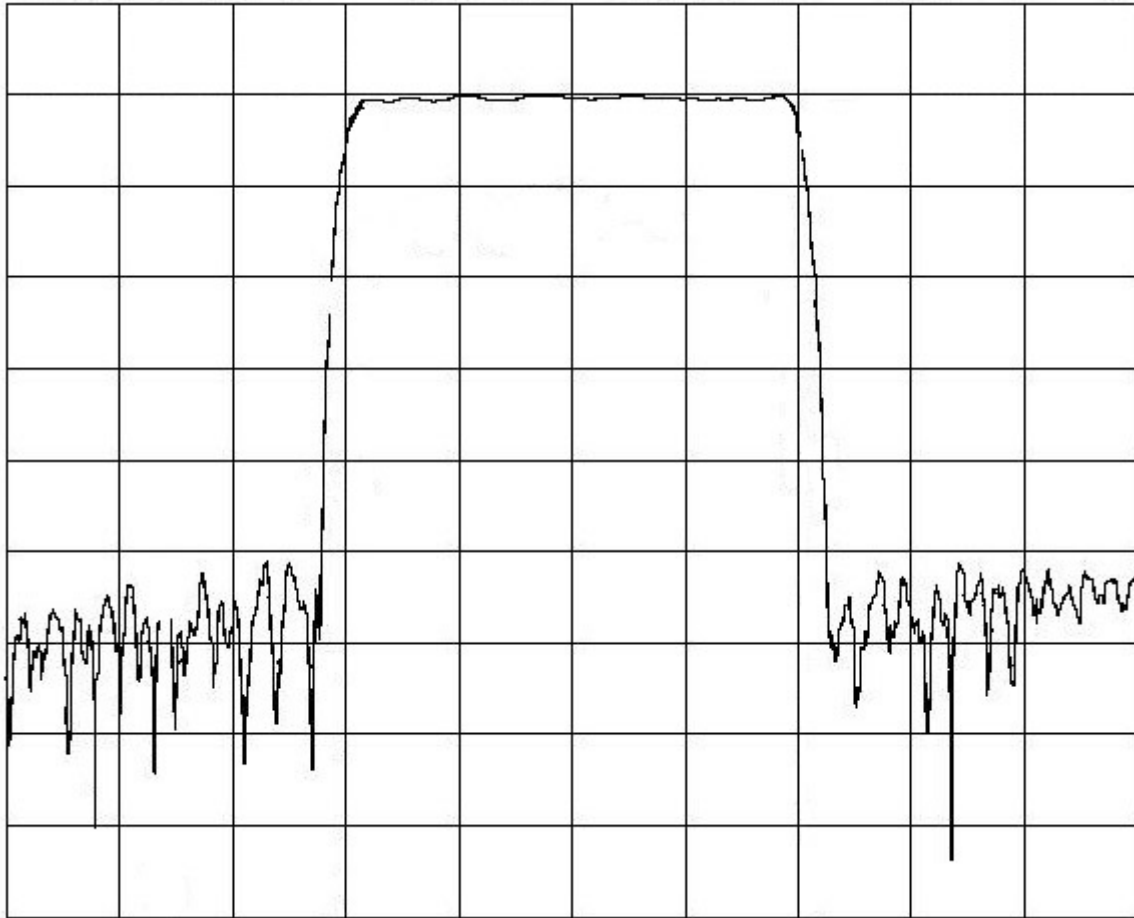
Vertical: 10dB/Div. Horizontal: 5 MHz/Div.
