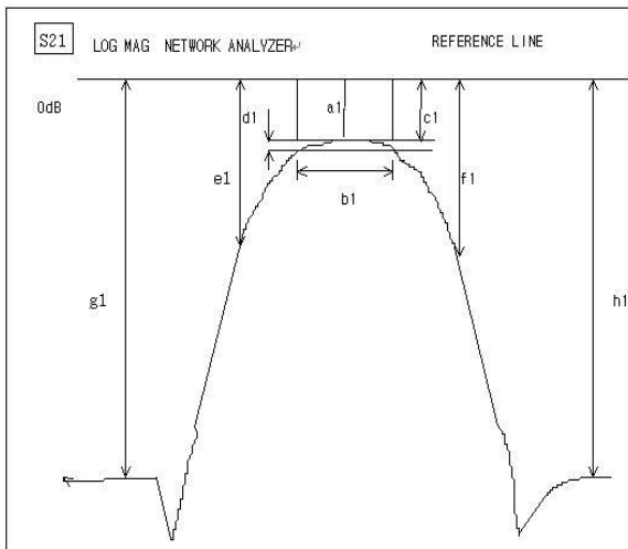
S21 LOG MAG NETWORK ANALYZER
