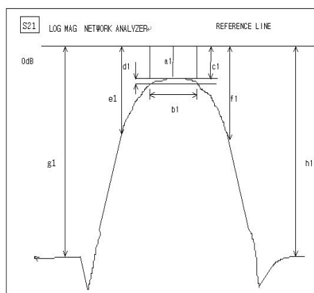
S21 LOG MAG NETWORK ANALYZER
