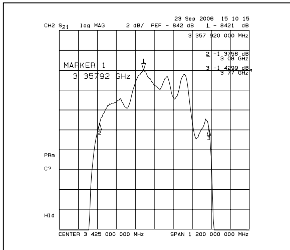
S21( ATTENUATION)
