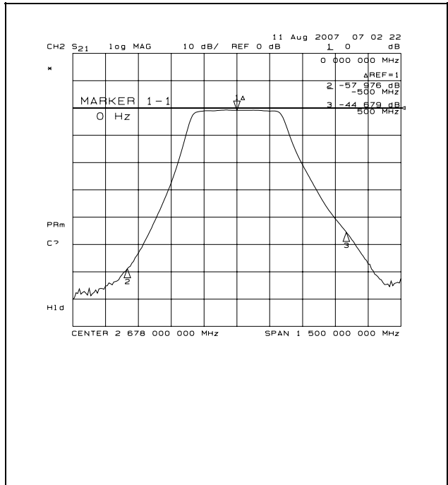
S21 (ATTENUATION)
