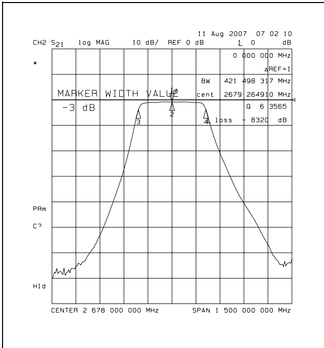
S21 (3.0DB BAND WIDTHS)
