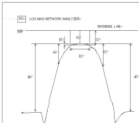
S21 LOG MAG NETWORK ANALYZER
