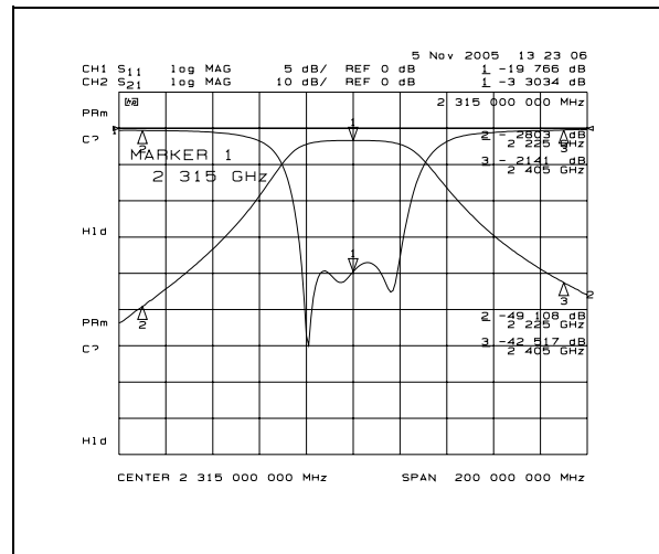
S21 &amp; S11 (3dB BAND WIDTH)
