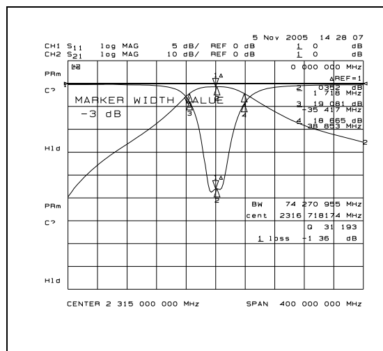
S21 & S11 (3dB BAND WIDTH)
