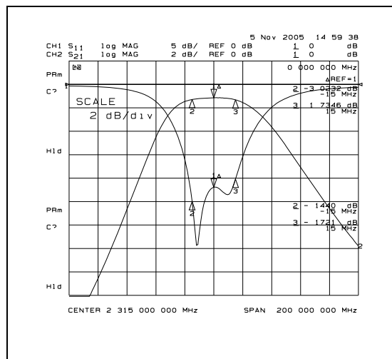
S21 & S11 (ATTENUATION)
