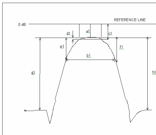
S21 & S11 (INSERTION LOSS, RETURN LOSS, ATTENUATION )
