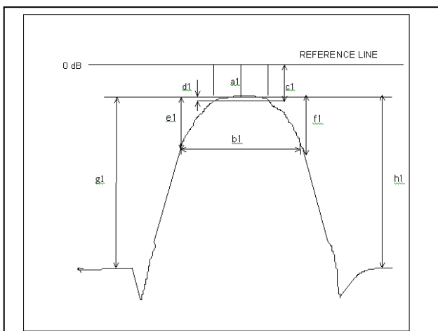
S21 LOG MAG NETWORK ANALYZER
