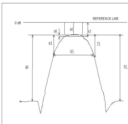
S21 LOG MAG NETWORK ANALYZER
