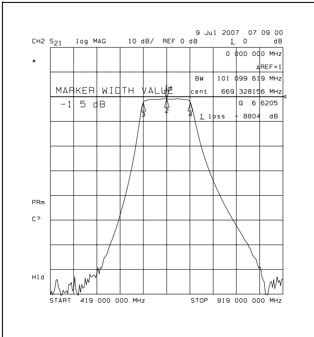
S21 (1.5DB BAND WIDTHS) (ATTENUATION)
